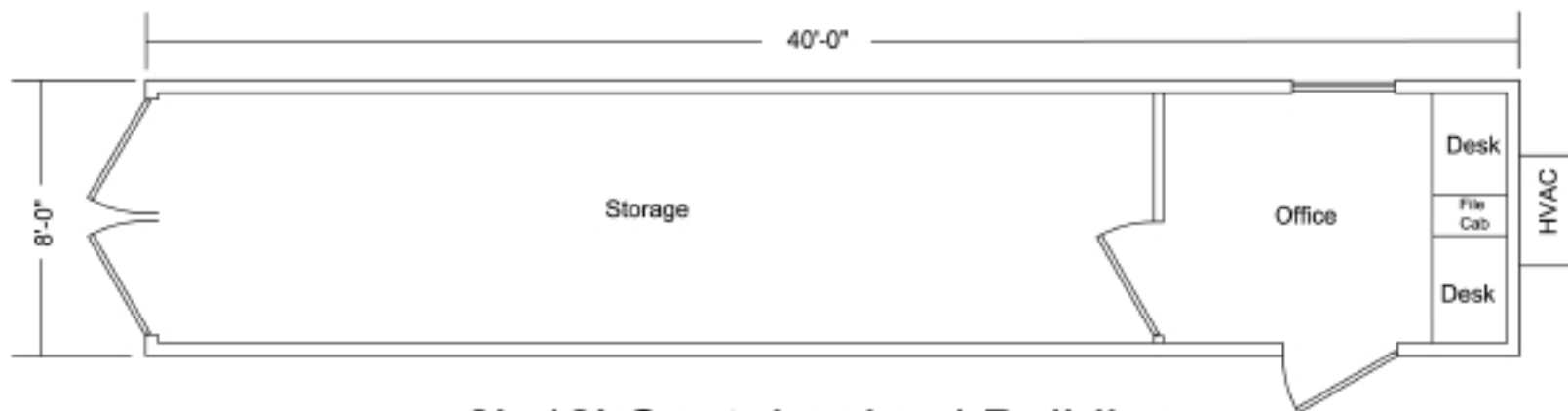
8'x40' Containerized Building
