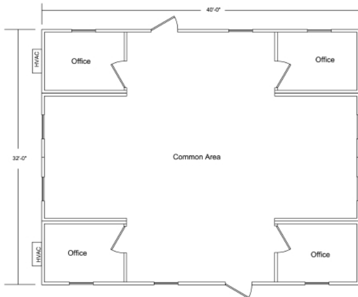
32x40 Ground Level Containerized Complex
