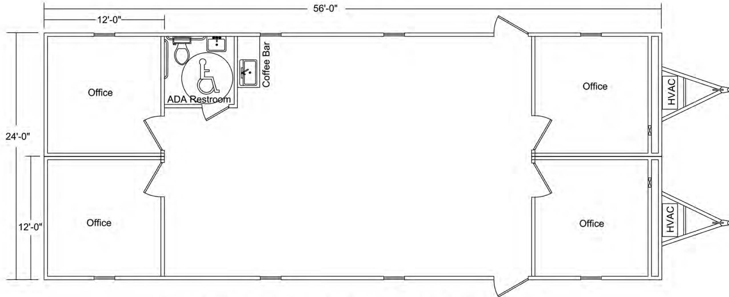
24x56 Mobile Office with ADA Restroom
